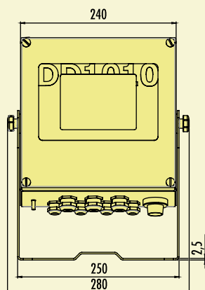
DD1010i desk-stand version
