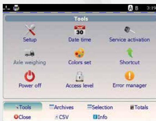
Navigation menu
